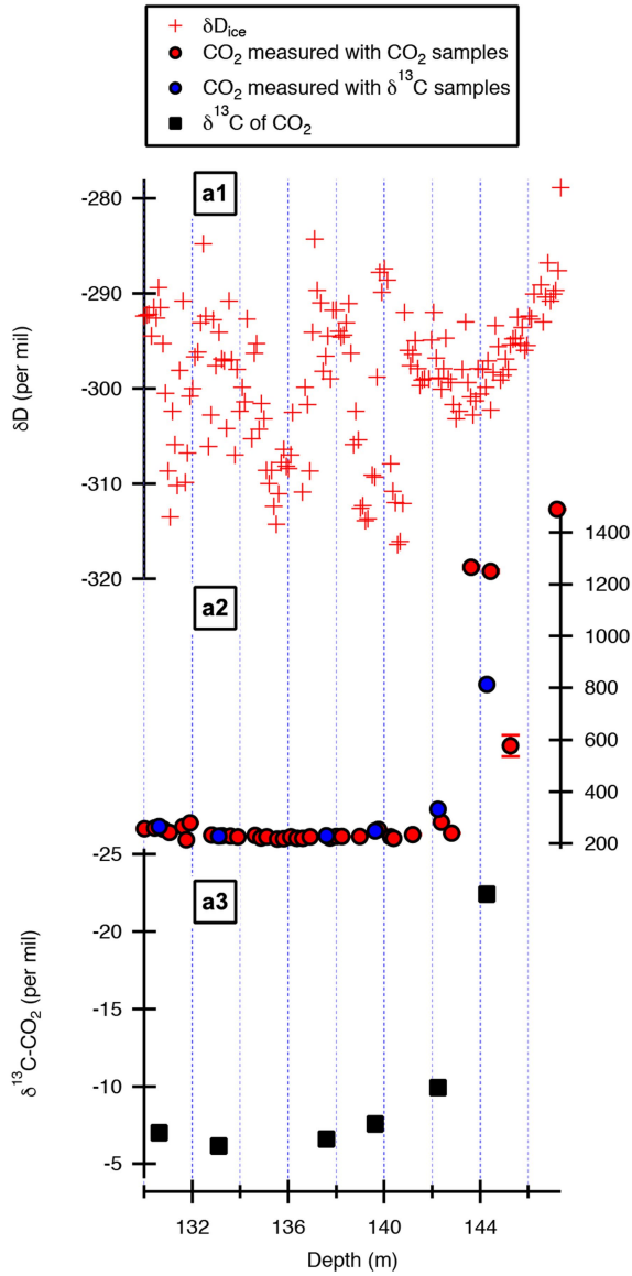
Extended Data Fig. 10 | Respiration in basal ice revealed by \delta^{13}C of CO_2 in ALHIC1503 and ALHIC1502. a, ALHIC1503; b, ALHIC1502. \delta D_{ice} (top), CO_2 (middle), and \delta^{13}C of CO_2 (bottom) in Allan Hills ice cores are plotted against depth. \delta D_{ice} and CO_2 (both measured independently in smaller samples,
