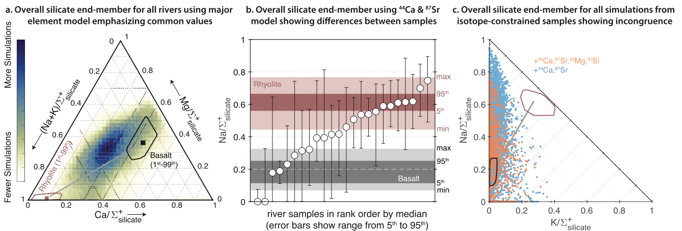
Figure 8. Inversion constrained composition of the silicate end-member. (a) Ternary diagram of the proportions of Na + K, Ca, and Mg. The MEANDIR results using only major element data are represented as a 2D histogram where darker colors reflect more simulations from each sample producing an end-member composition with that particular value. For comparison, we show the compositions of basalts and rhyolites as black and light red squares with outlines that encompass 98% of the measured variability. The gray line connecting the black and light red squares is the mixing line between mean basalt and mean rhyolite. (b) Inversion constrained values for the Na/\Sigma^+ using Ca and Sr isotopic data as model constraints. The white circles show the median values calculated using the model and the error bars show the range from the 5th to 95th percentiles. For comparison, we show the minimum/maximum (light shading) and 5th/95th percentile (dark shading) ranges of Na/\Sigma^+ for Icelandic basalts (black) and rhyolites (light red). (c) Incongruent release of Na relative to K evident in the isotope-constrained solute mass balance model simulations. The blue (Ca and Sr isotope constrained; n = 24 ) and orange (Mg, Si, Ca, and Sr isotope constraints; n = 7 ) points show the predicted composition of the silicate end-member for each individual simulation for all rivers considered. Similar results (i.e., incongruent release of Na relative to K) are also obtained using only major elements as constraints.
