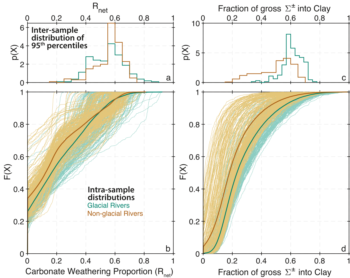
Figure 12. Solute mass balance model predictions for glaciated versus non-glaciated watersheds. (a) Inter-sample distribution of 95th percentile values for the proportion of carbonate weathering ( R_{net} ) for glaciated (blue) and non-glaciated (brown) river samples. (b) Full distributions of R_{net} for all glacial and non-glacial river samples. The thin, lighter-colored lines show individual samples whereas the thicker, darker-colored lines show the distributions for all samples combined. Panel (c) same as in panel (a), but showing the inter-sample distributions for the fraction of \Sigma^{\pm} + \text{SO}_4 uptake into clays ( F_{clay}^{\Sigma^{\pm}} ). Panel (d) same as in panel (b) but showing the full distributions of F_{clay}^{\Sigma^{\pm}} for glaciated and non-glaciated watersheds.
